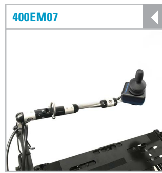
400EM07 Link-It to Midline Swing-Away Joystick Mount
