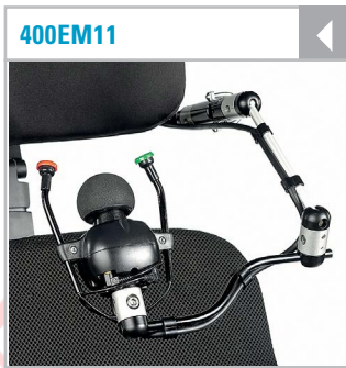
400EM11 Link-It to Headrest, Swing-Away
