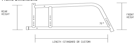
Frame Dimensions
